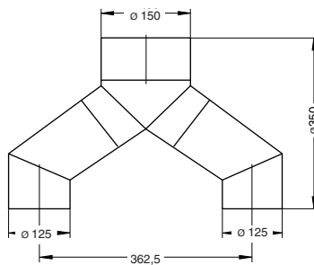
Ducting kit (dimensions)
